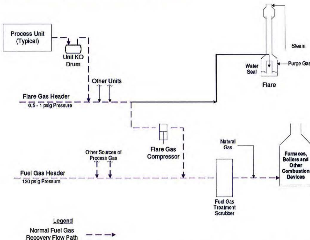
Figure 4-2 – Typical Fuel Gas Recovery System
