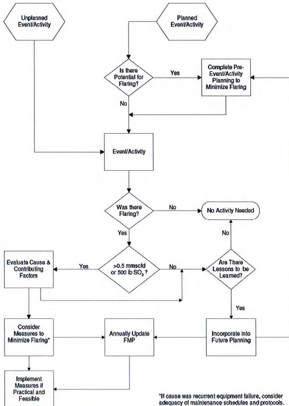
Figure 1-2 – Flare Minimization Flowchart
