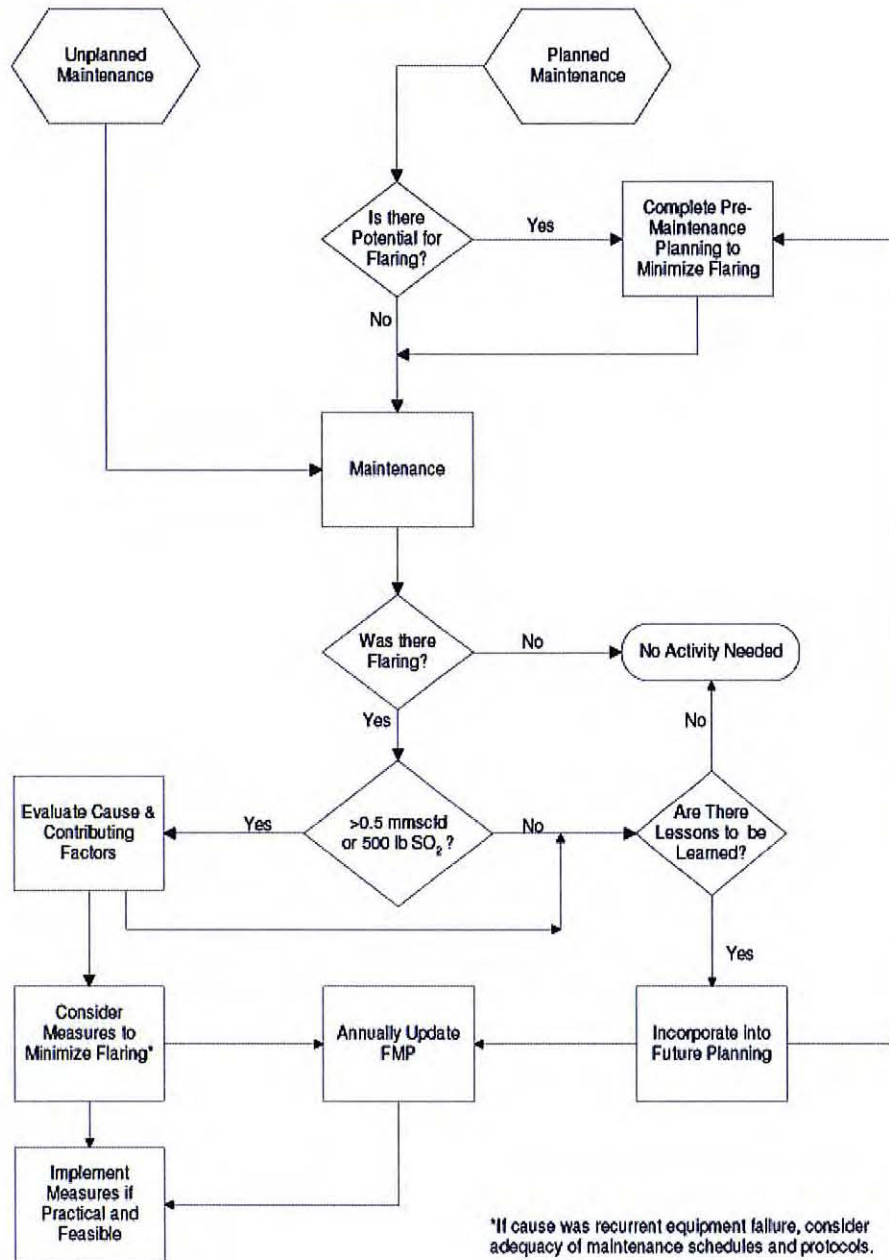
Figure 4-1 – Flare Minimization Flowchart for Maintenance
