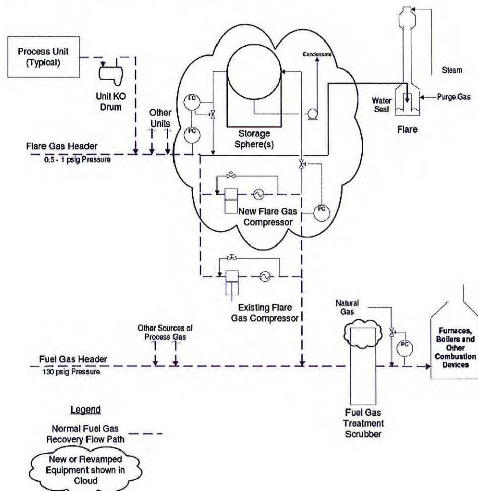
Figure 4-3 – Flare Gas Recovery System
