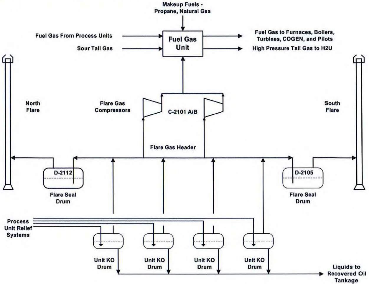
Figure 1-3 – Flare Gas Recovery System
