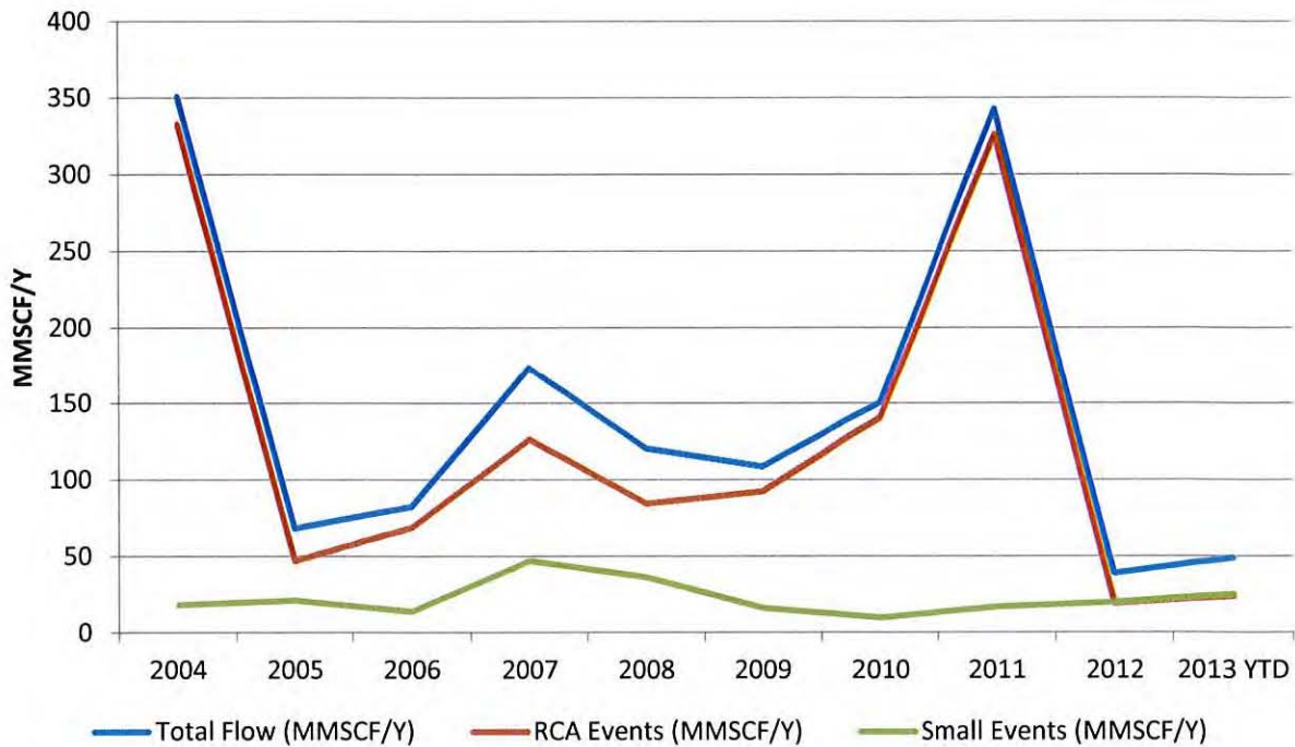
Figure 0-3 – Flare Vent Gas Volume Comparison
