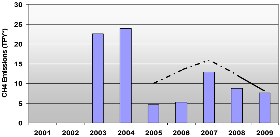
Methane Emissions
