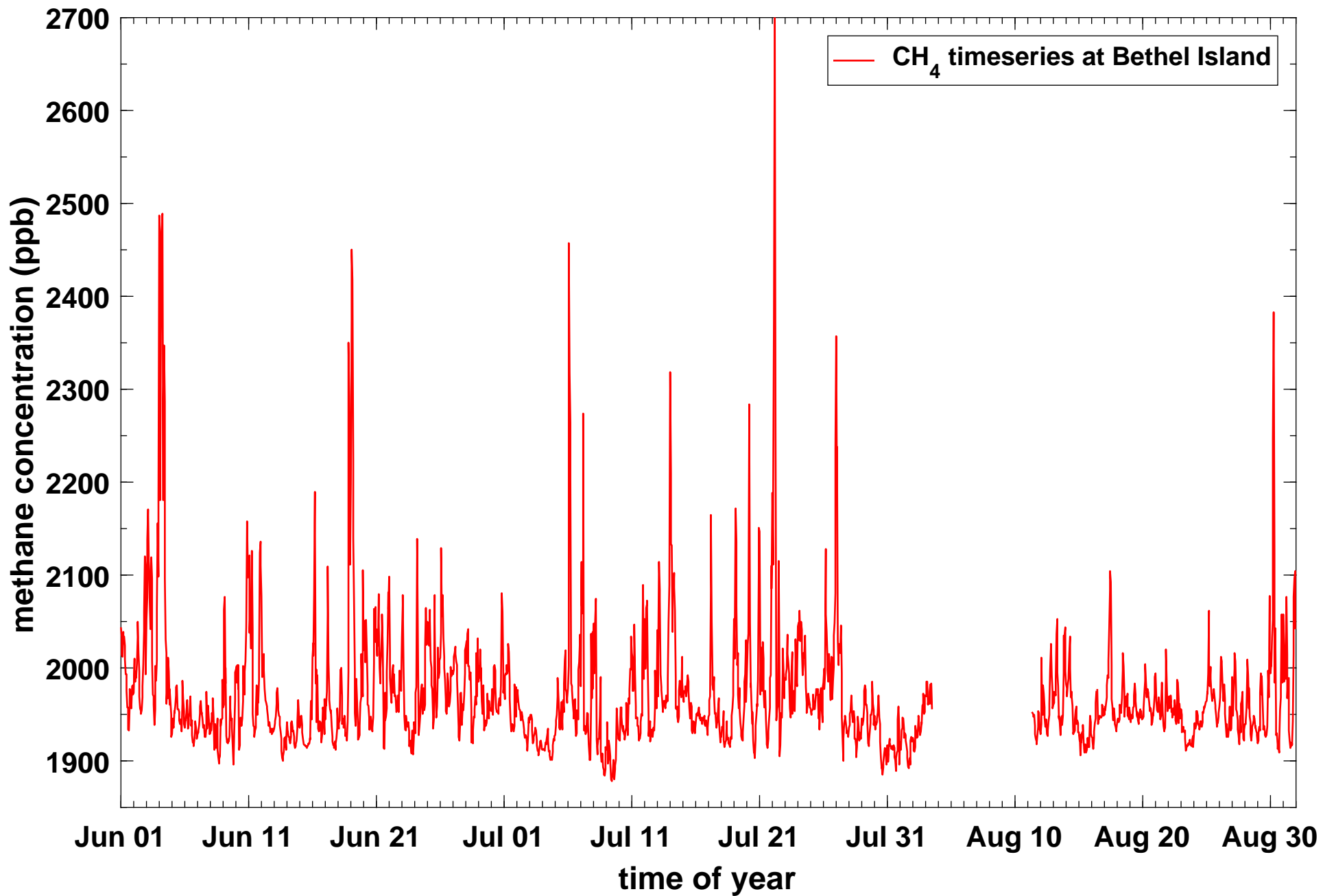
Timeseries of hourly CH 4 concentrations (in ppb) at Bethel Island during summer 2016 (Jun 1 - Aug 31).
