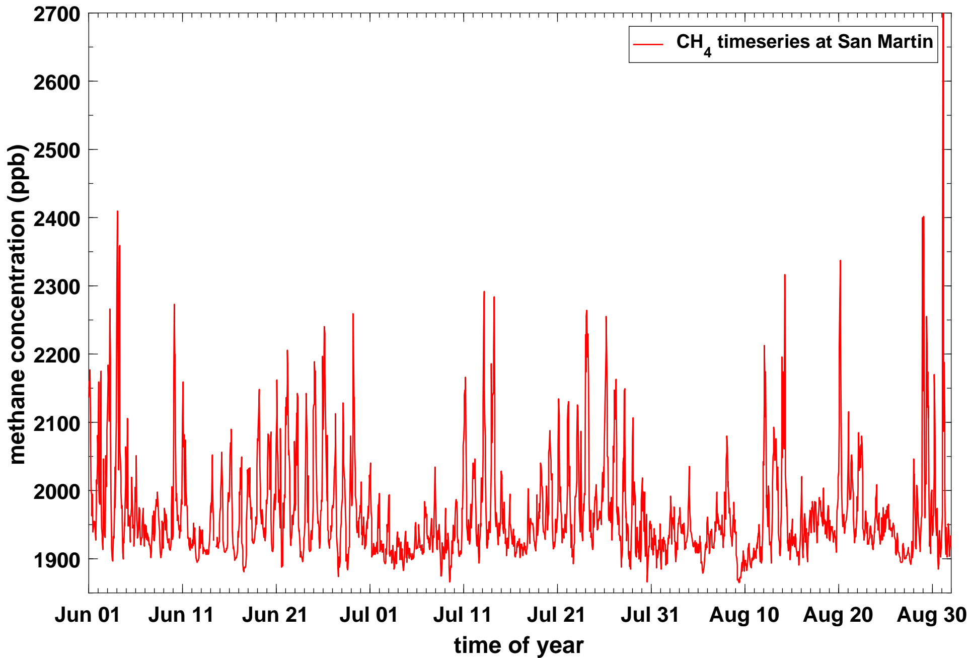
Timeseries of hourly CH 4 concentrations (in ppb) at San Martin during summer 2016 (Jun 1 - Aug 31).
