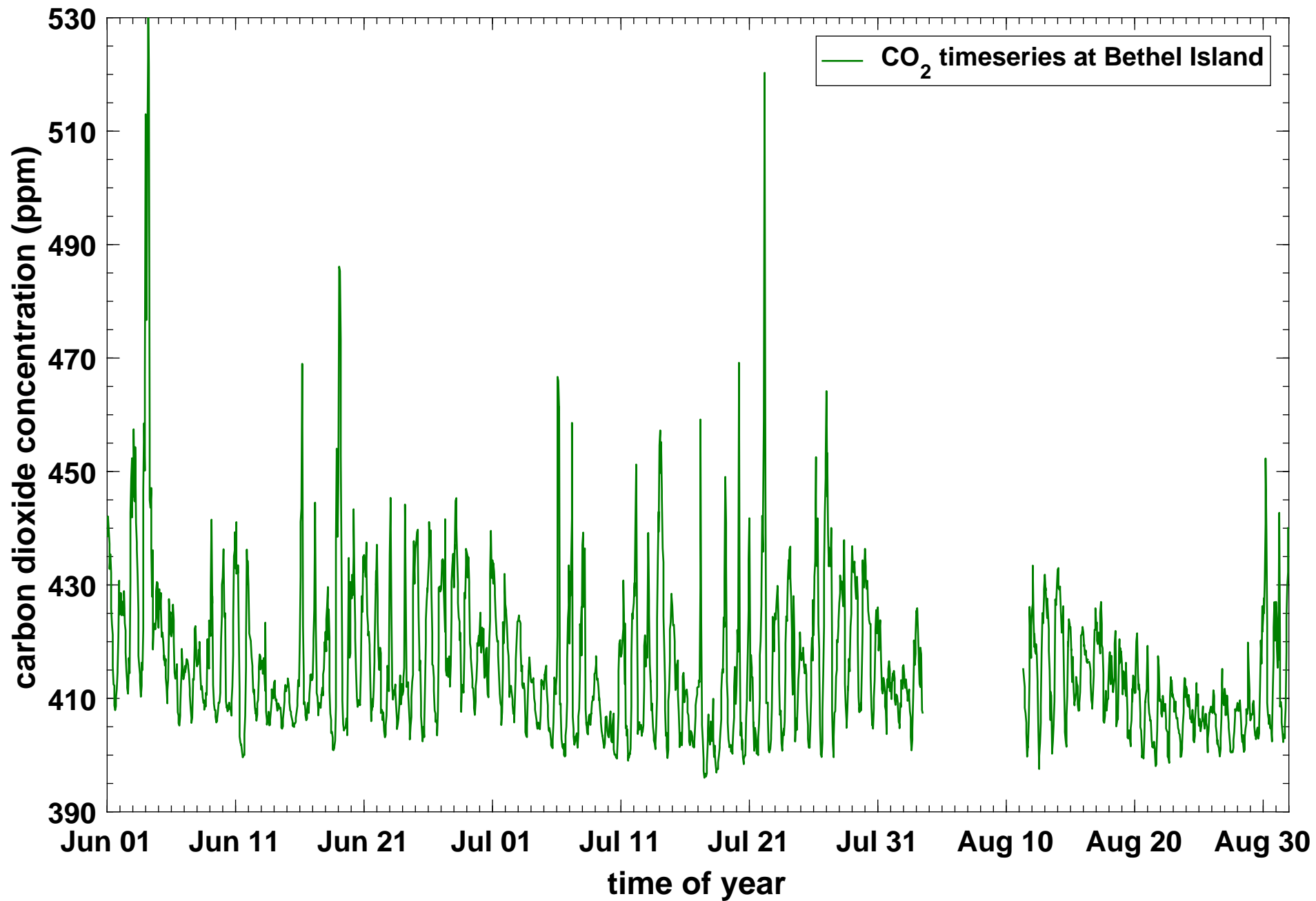
Timeseries of hourly CO 2 concentrations (in ppm) at Bethel Island during summer 2016 (Jun 1 - Aug 31).
