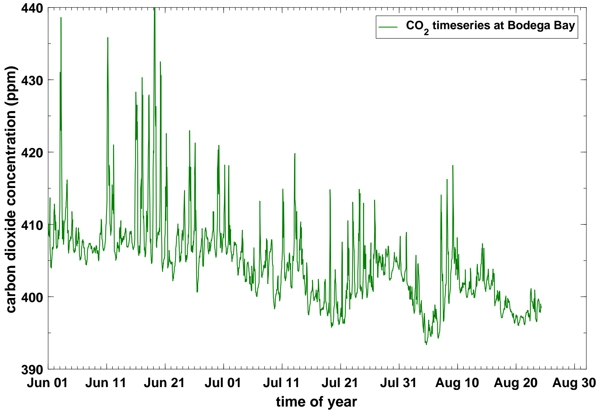
Timeseries of hourly CO 2 concentrations (in ppm) at Bodega Bay during summer 2016 (Jun 1 - Aug 31).
