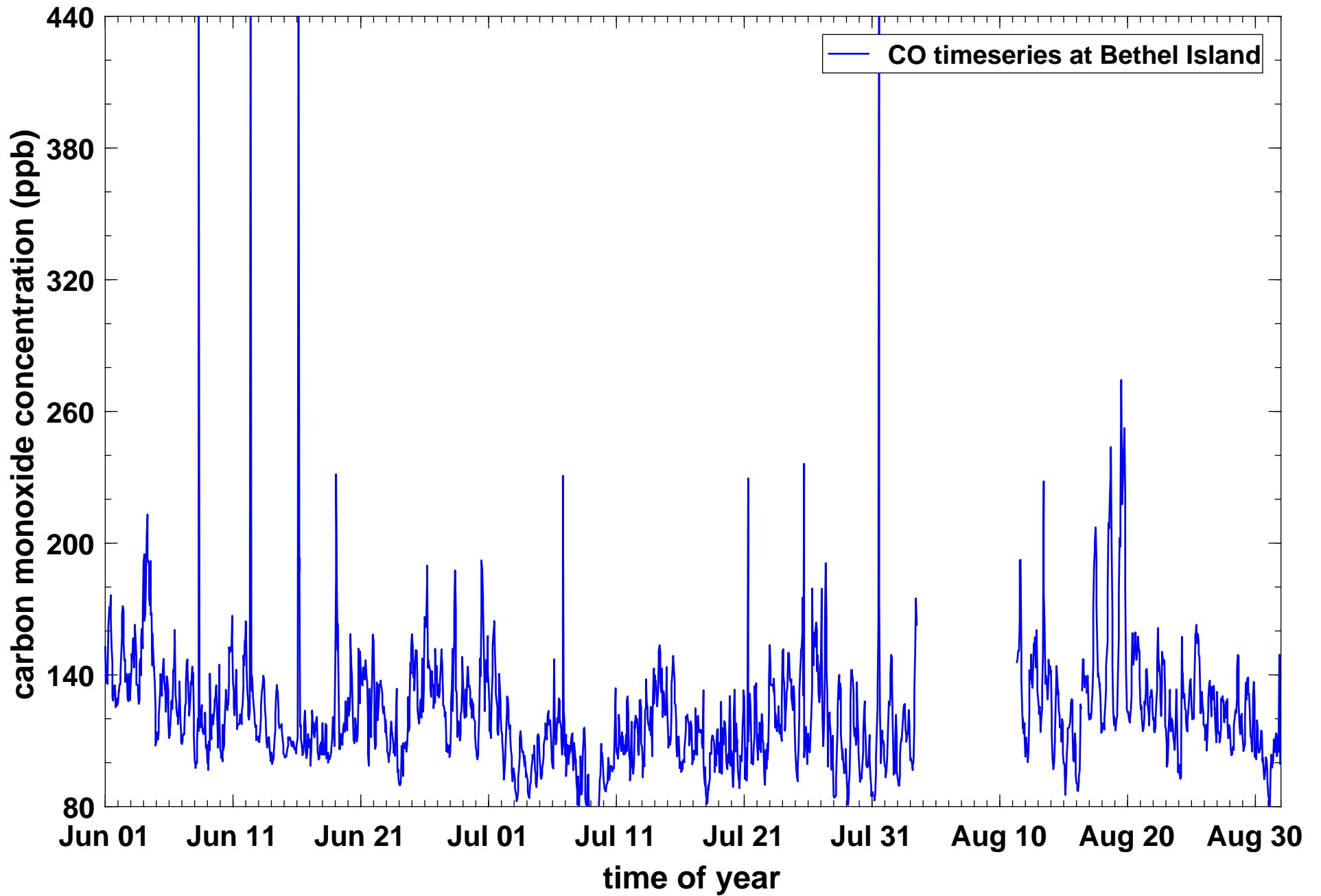
Timeseries of hourly CO concentrations (in ppb) at Bethel Island during summer 2016 (Jun 1 - Aug 31).
