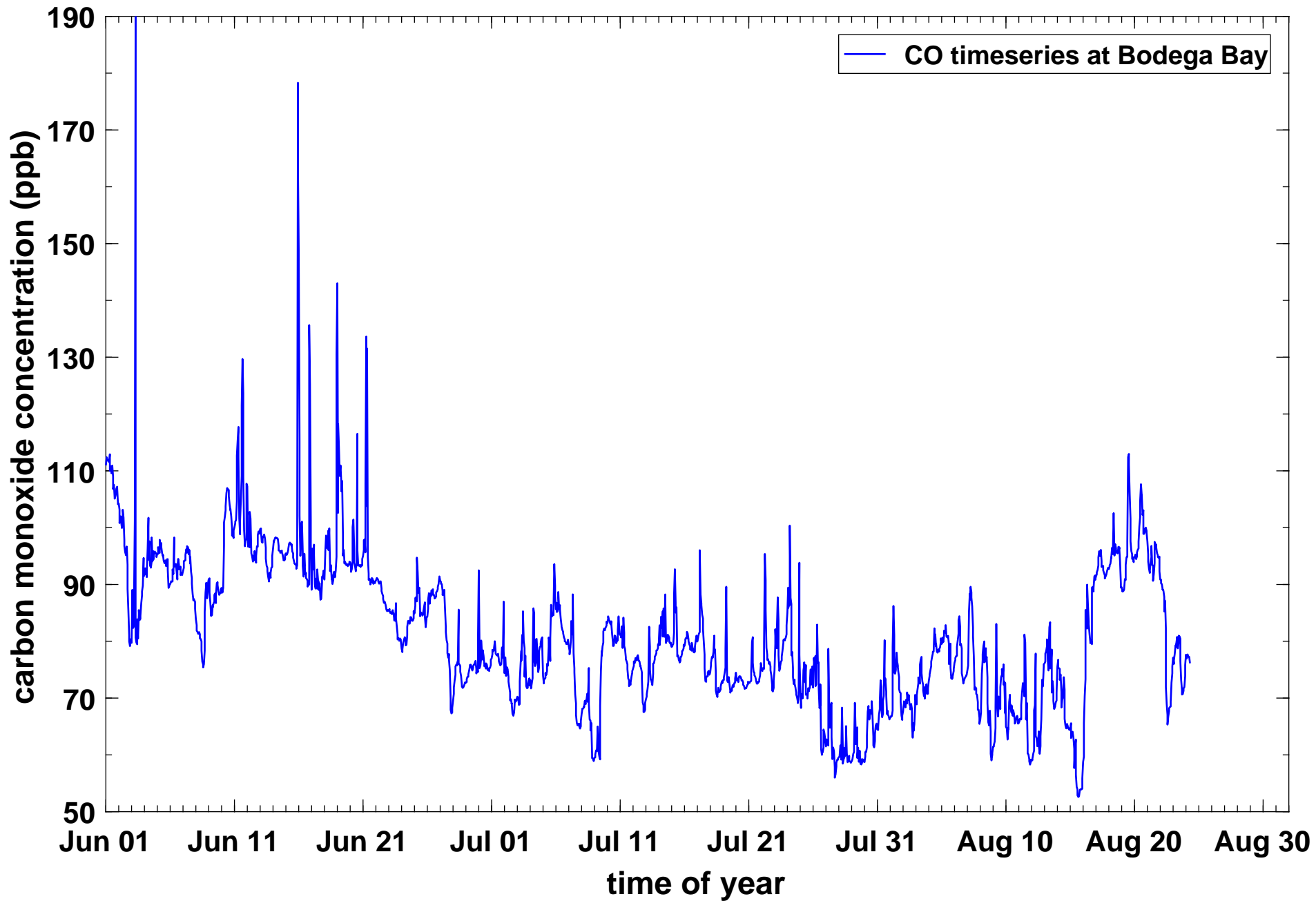
Timeseries of hourly CO concentrations (in ppb) at Bodega Bay during summer 2016 (Jun 1 - Aug 31).
