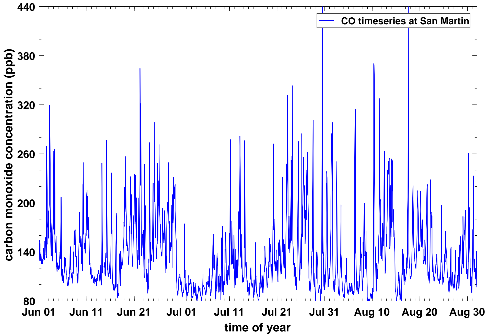
Timeseries of hourly CO concentrations (in ppb) at San Martin during summer 2016 (Jun 1 - Aug 31).
