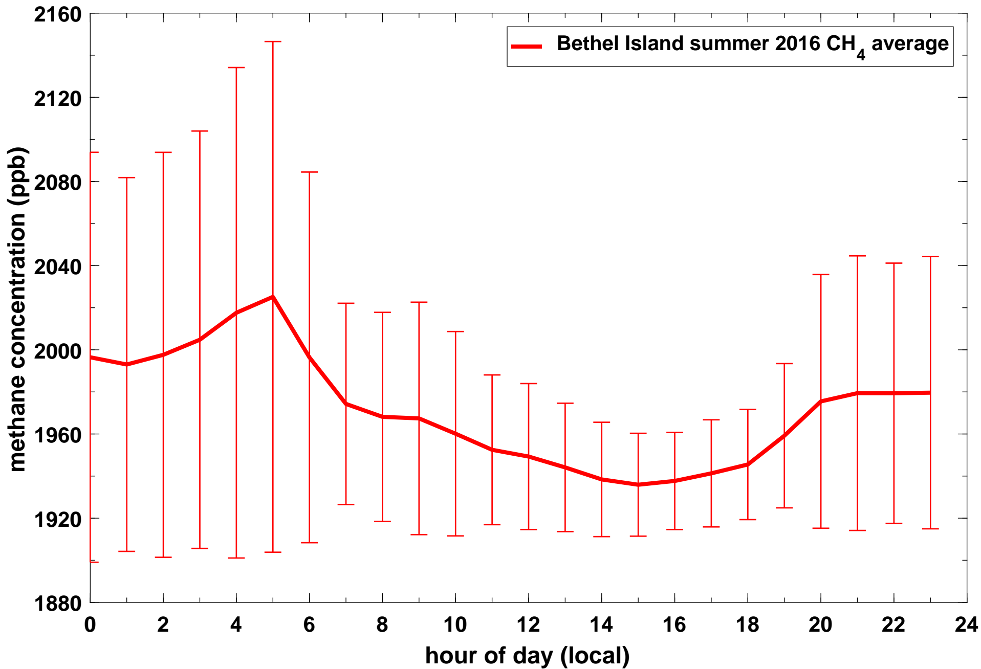
Average daily concentration profile of CH 4 (in ppb) at Bethel Island during summer 2016 (Jun 1 - Aug 31). The solid line denotes hourly averages for the entire season while the whiskers denote one standard deviation of the data values for each hour.
