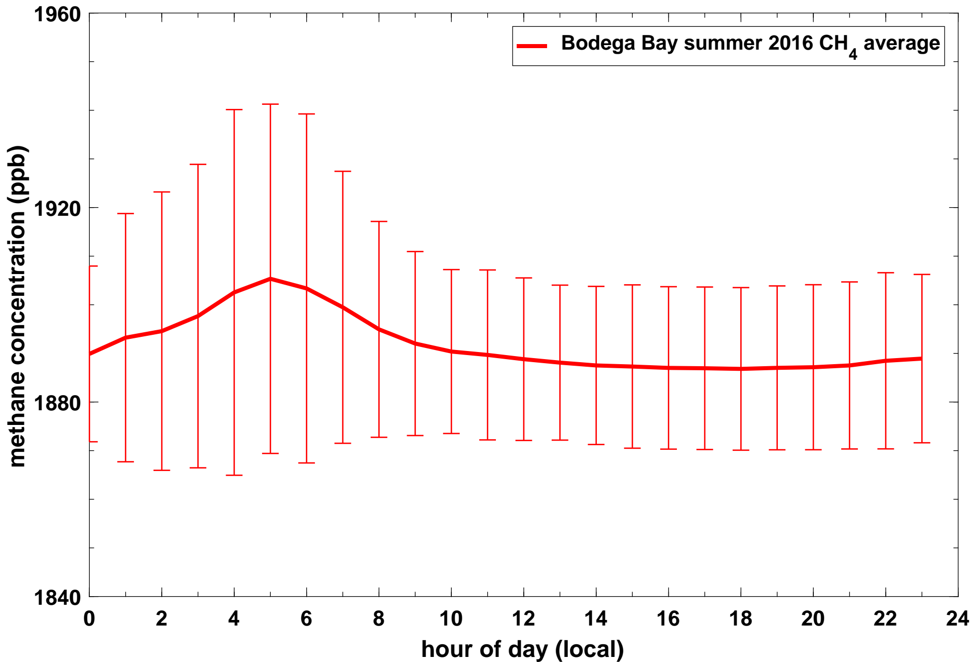
Average daily concentration profile of CH 4 (in ppb) at Bodega Bay during summer 2016 (Jun 1 - Aug 31). The solid line denotes hourly averages for the entire season while the whiskers denote one standard deviation of the data values for each hour.
