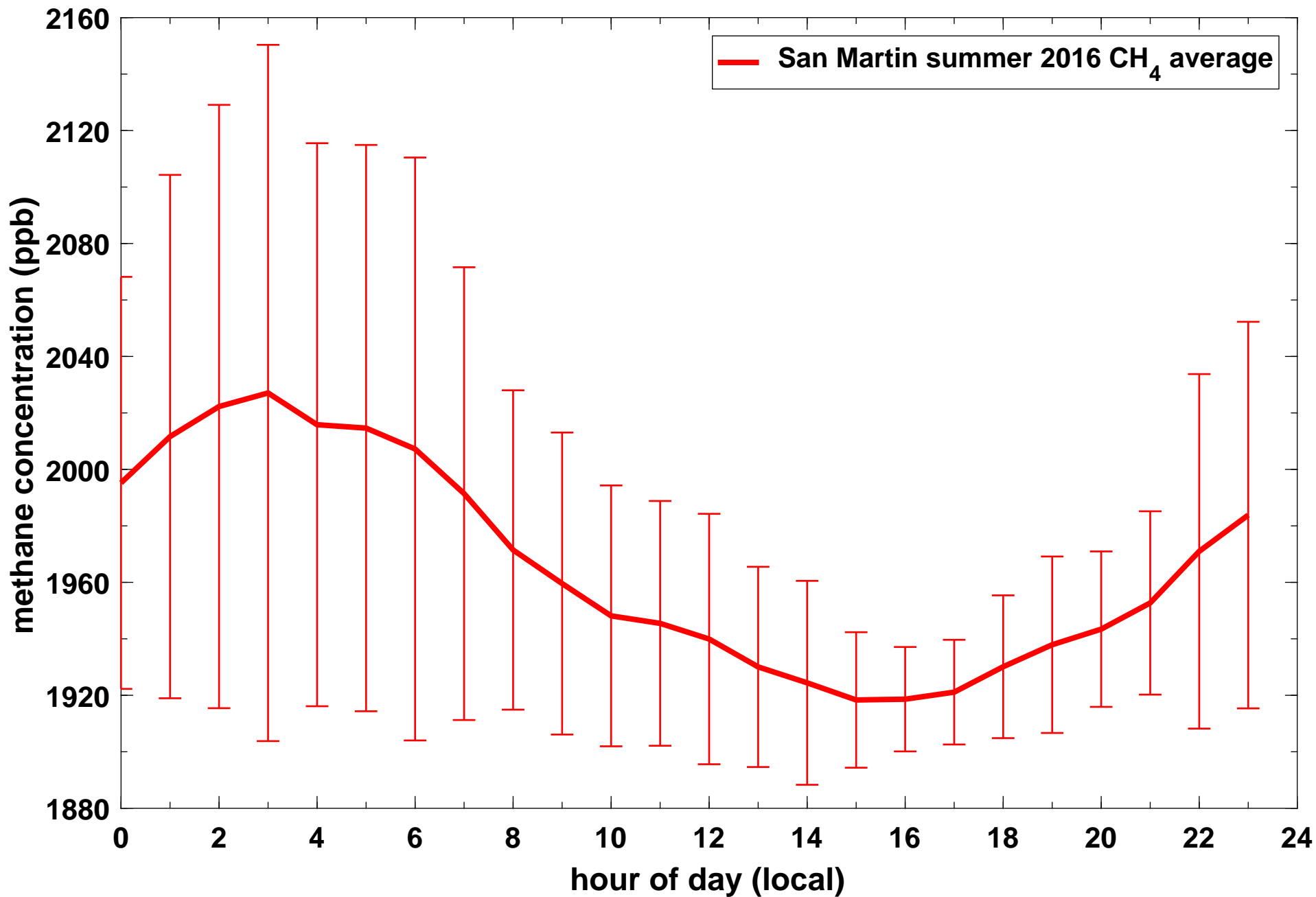
Average daily concentration profile of CH 4 (in ppb) at San Martin during summer 2016 (Jun 1 - Aug 31). The solid line denotes hourly averages for the entire season while the whiskers denote one standard deviation of the data values for each hour.
