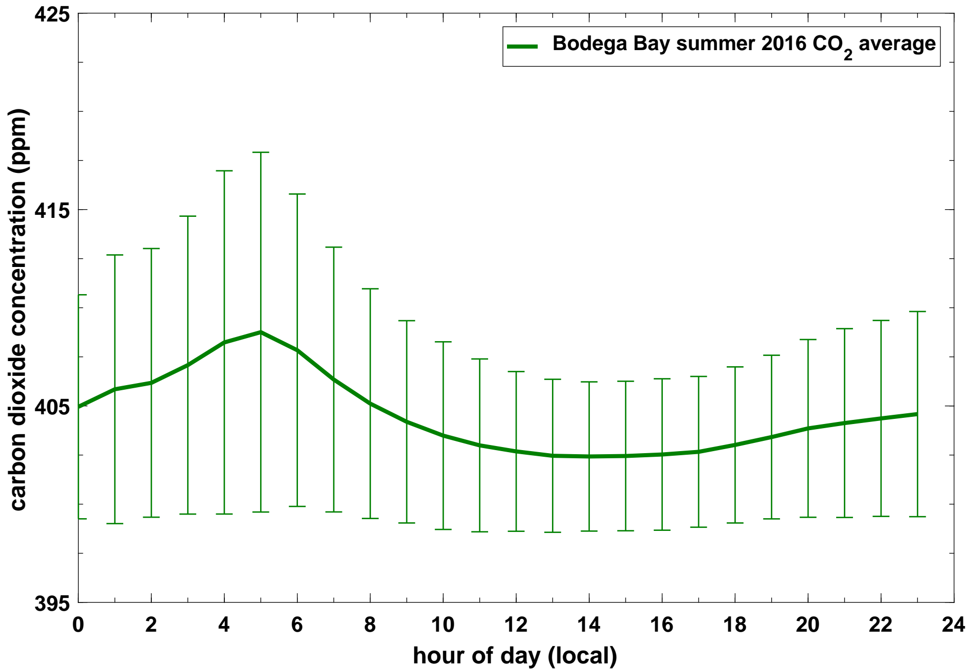
Average daily concentration profile of CO 2 (in ppm) at Bodega Bay during summer 2016 (Jun 1 - Aug 31). The solid line denotes hourly averages for the entire season while the whiskers denote one standard deviation of the data values for each hour.
