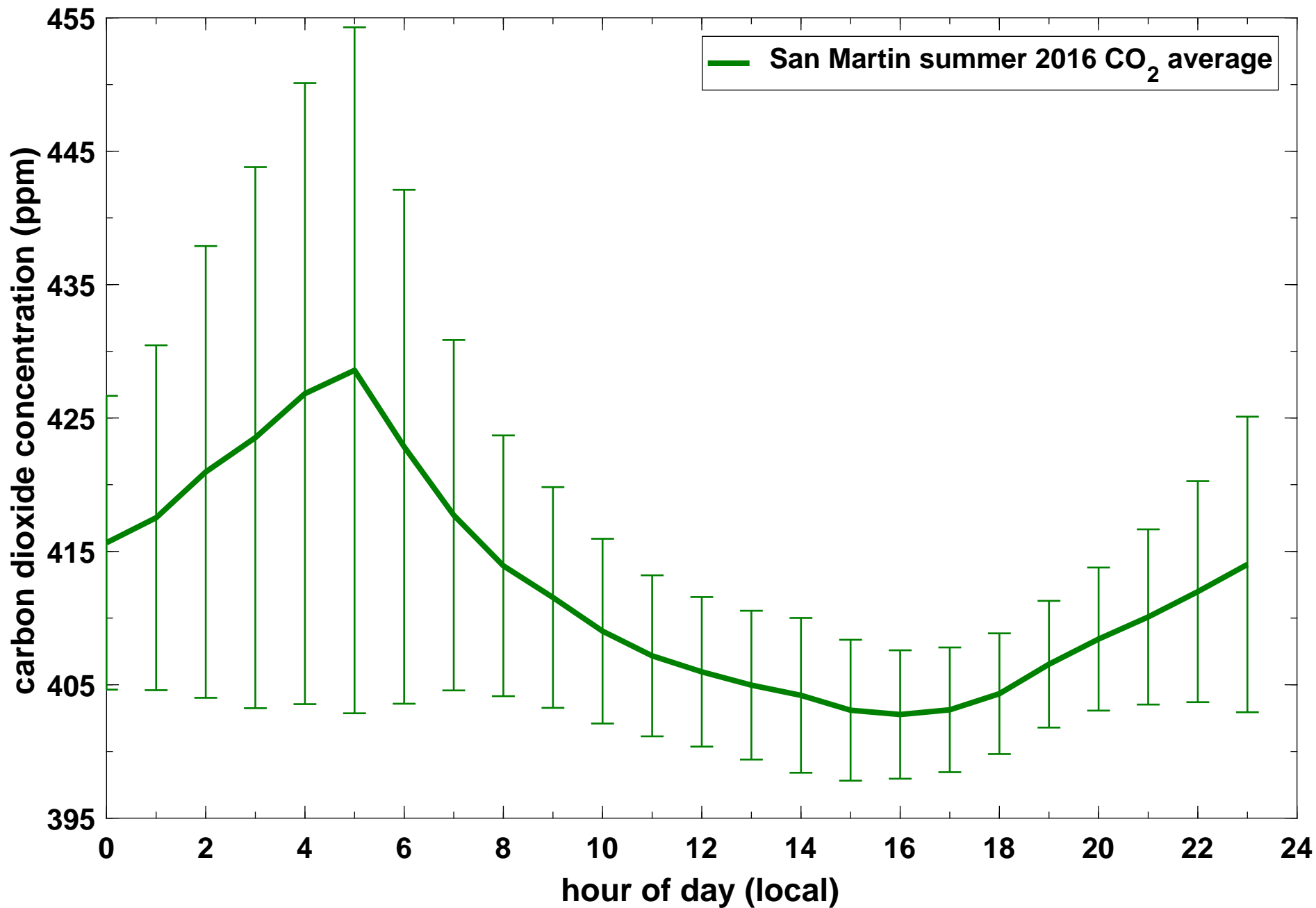
Average daily concentration profile of CO 2 (in ppm) at San Martin during summer 2016 (Jun 1 - Aug 31). The solid line denotes hourly averages for the entire season while the whiskers denote one standard deviation of the data values for each hour.
