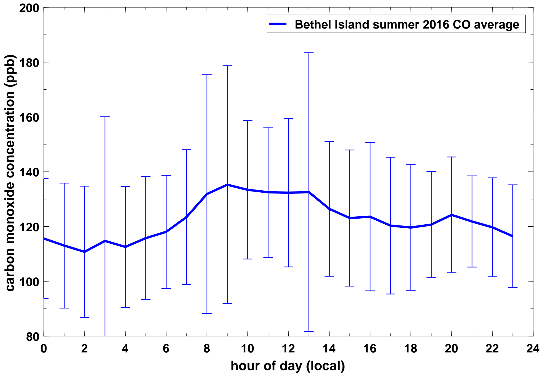
Average daily concentration profile of CO (in ppb) at Bethel Island during summer 2016 (Jun 1 - Aug 31). The solid line denotes hourly averages for the entire season while the whiskers denote one standard deviation of the data values for each hour.
