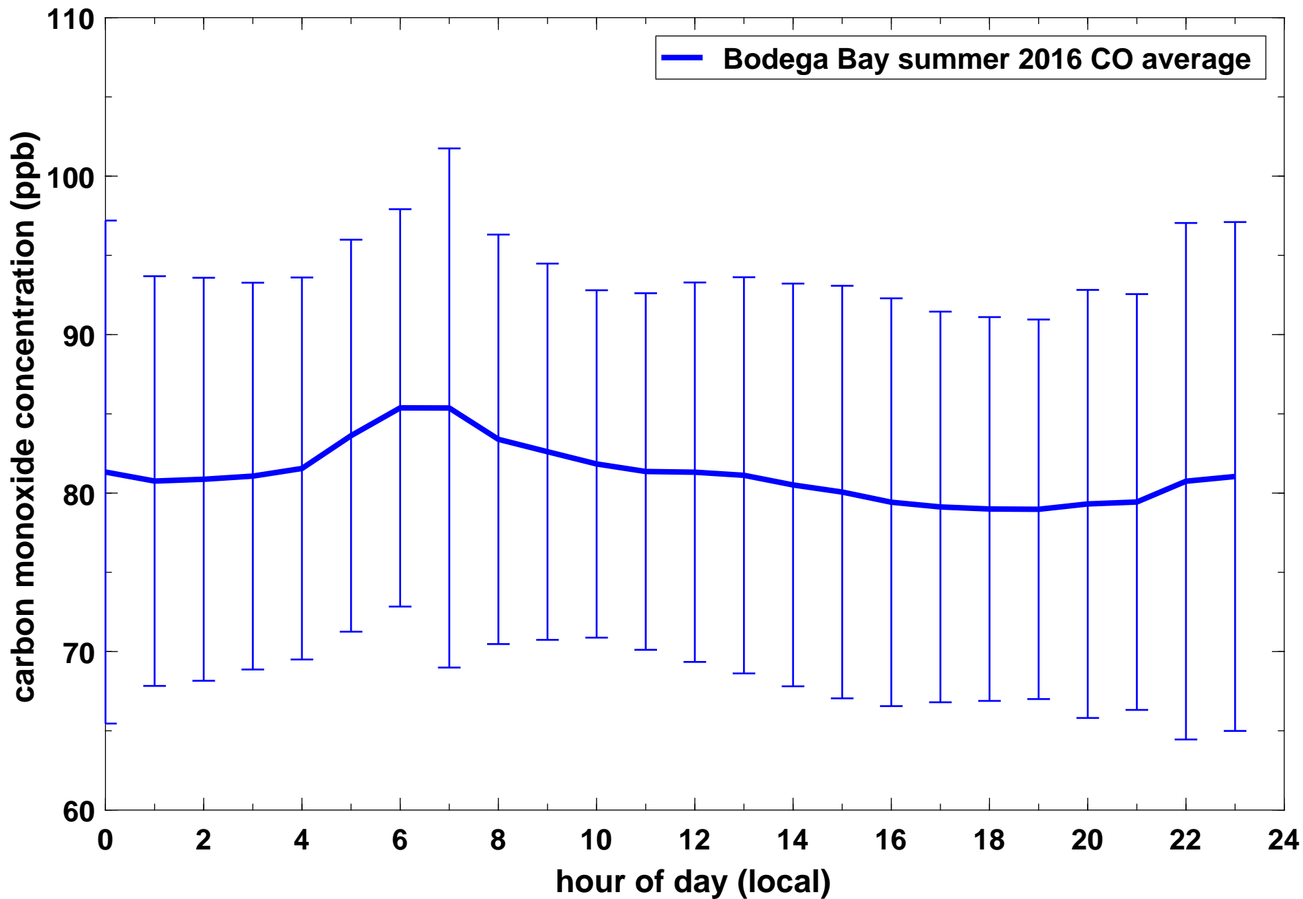
Average daily concentration profile of CO (in ppb) at Bodega Bay during summer 2016 (Jun 1 - Aug 31). The solid line denotes hourly averages for the entire season while the whiskers denote one standard deviation of the data values for each hour.
