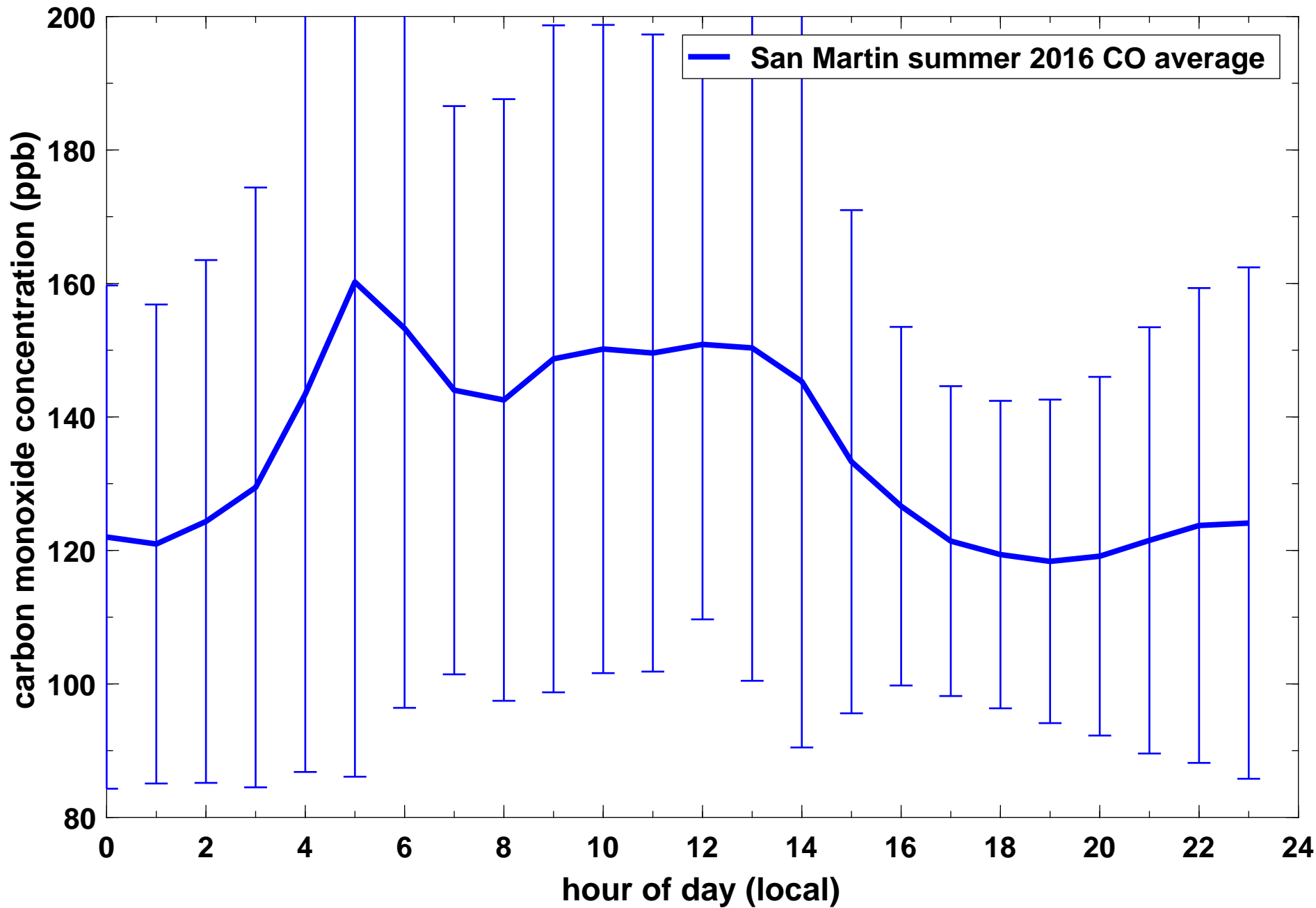
Average daily concentration profile of CO (in ppb) at San Martin during summer 2016 (Jun 1 - Aug 31). The solid line denotes hourly averages for the entire season while the whiskers denote one standard deviation of the data values for each hour.
