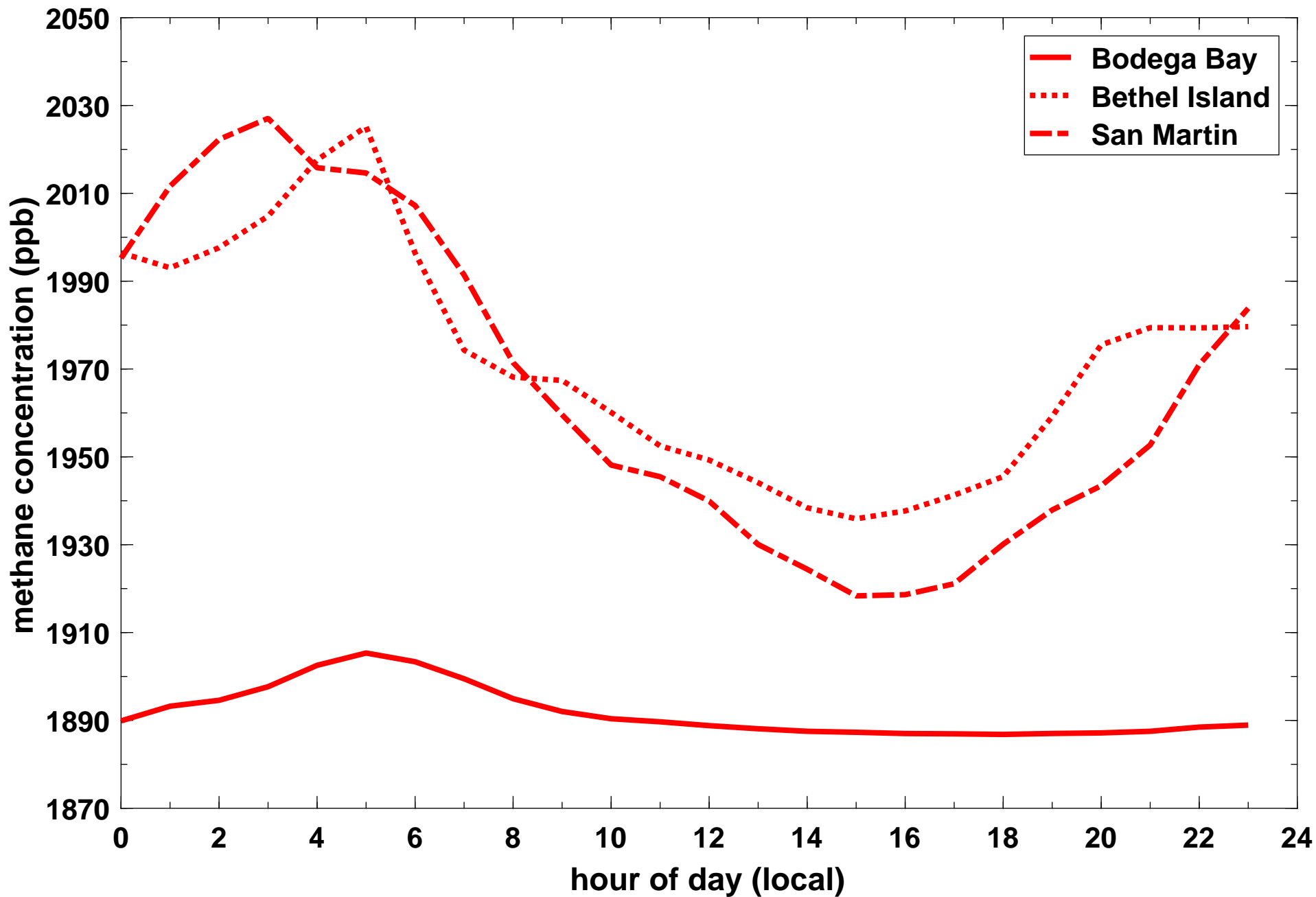
Average daily concentration profiles of CH 4 (in ppb) at Bodega Bay (solid line), Bethel Island (dotted line) and San Martin (dash-dot line) during summer 2016 (Jun 1 - Aug 31). The hourly data values represent averages over the entire season.
