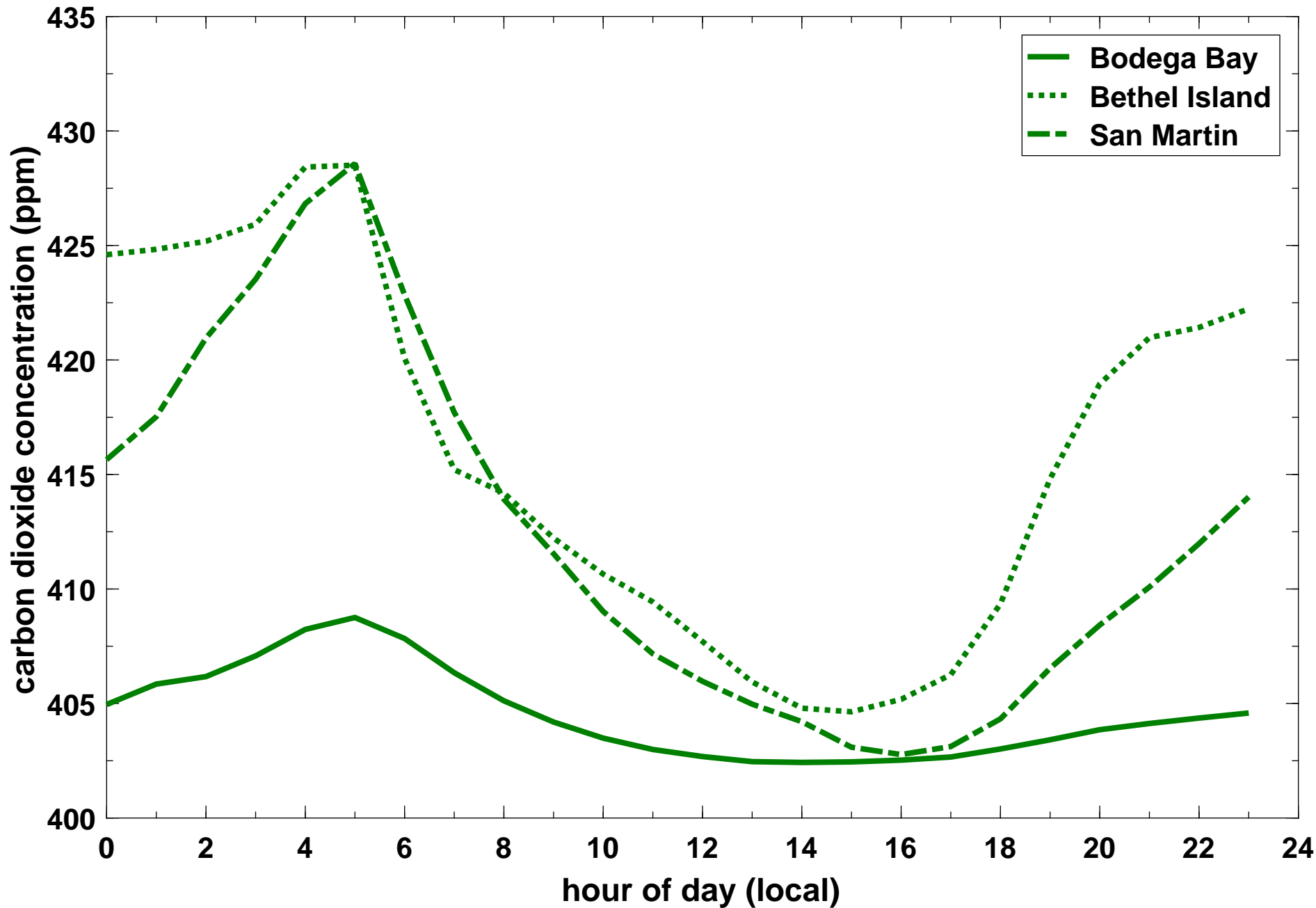
Average daily concentration profiles of CO 2 (in ppm) at Bodega Bay (solid line), Bethel Island (dotted line) and San Martin (dash-dot line) during summer 2016 (Jun 1 - Aug 31). The hourly data values represent averages over the entire season.
