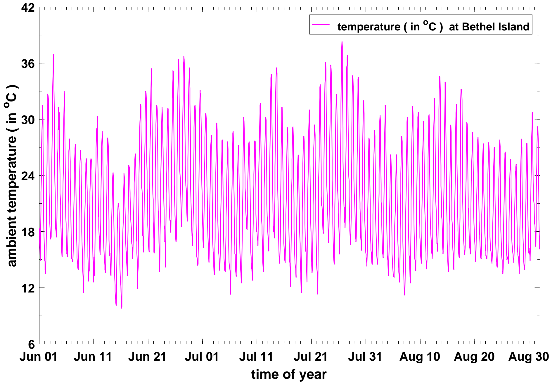
Timeseries of hourly-averaged air temperatures (in degree Celsius) at Bethel Island during summer 2016 (Jun 1 - Aug 31).
