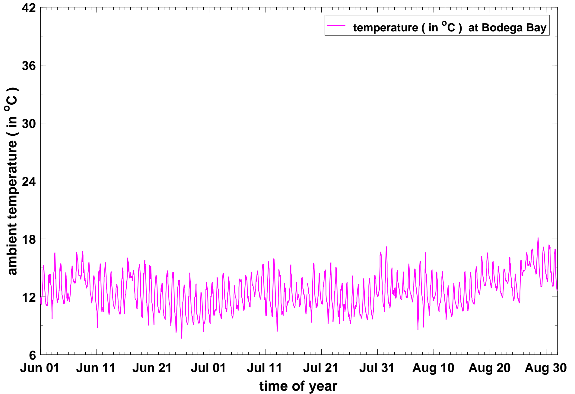
Timeseries of hourly-averaged air temperatures (in degree Celsius) at Bodega Bay during summer 2016 (Jun 1 - Aug 31).
