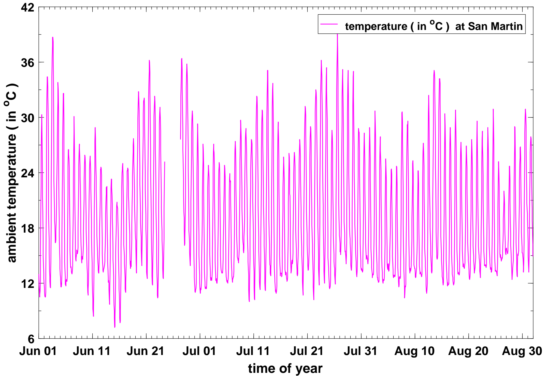
Timeseries of hourly-averaged air temperatures (in degree Celsius) at San Martin during summer 2016 (Jun 1 - Aug 31).
