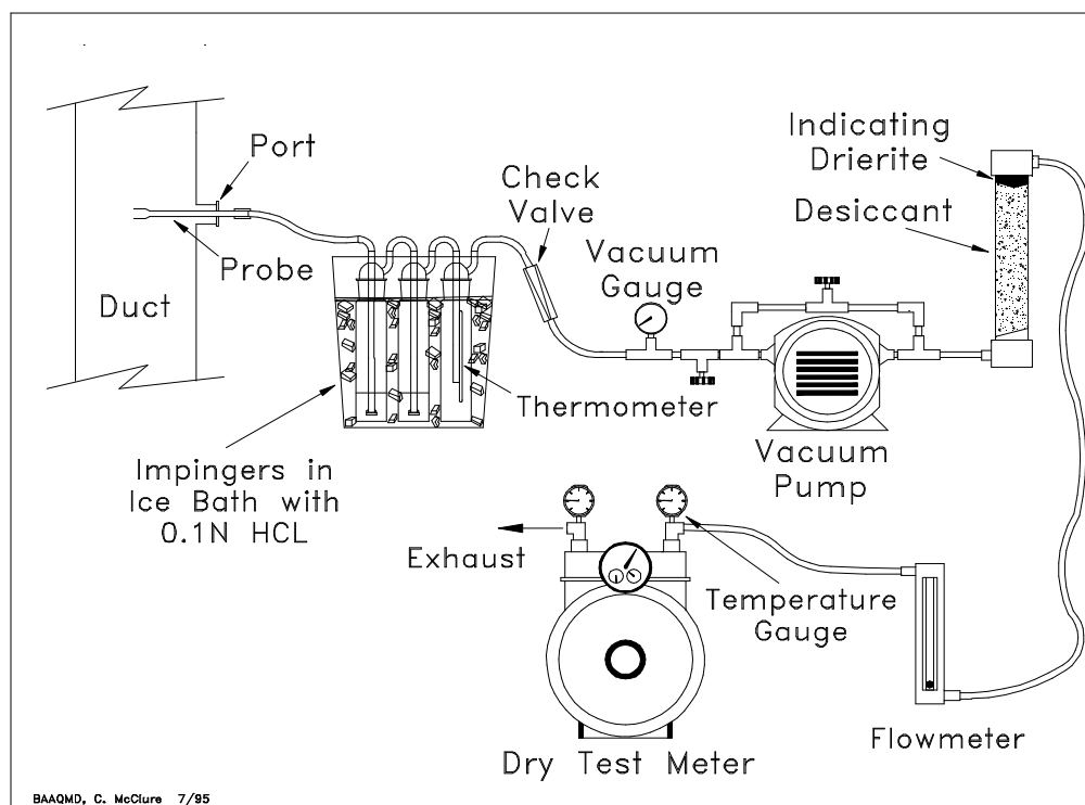
Trimethylamine Sampling Train
