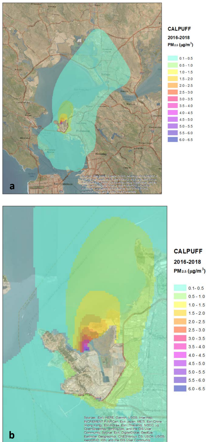
Figure ES.1: Three-year (2016–2018) average CALPUFF-simulated PM 2.5 concentrations for (a) the 100-m receptor domain, and (b) a zoomed-in area of high concentrations. Emissions from all (119) point sources are included in these simulations. Concentrations inside the Chevron fence line and that are below 0.1 µg/m 3 are not shown.
