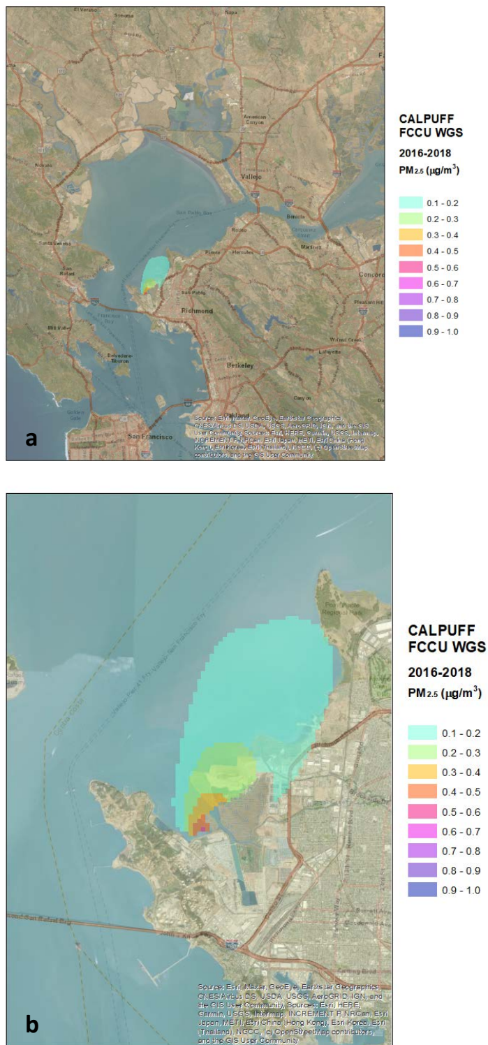
Figure ES.3: Three-year (2016–2018) average CALPUFF-simulated PM 2.5 concentrations for: (a) the 100-m receptor domain, and (b) a zoomed-in area of high concentrations. Emissions from the FCCU only (with an assumed WGS) are included in these simulations. Concentrations inside the Chevron fence line and that are below 0.1 µg/m 3 are not shown.
