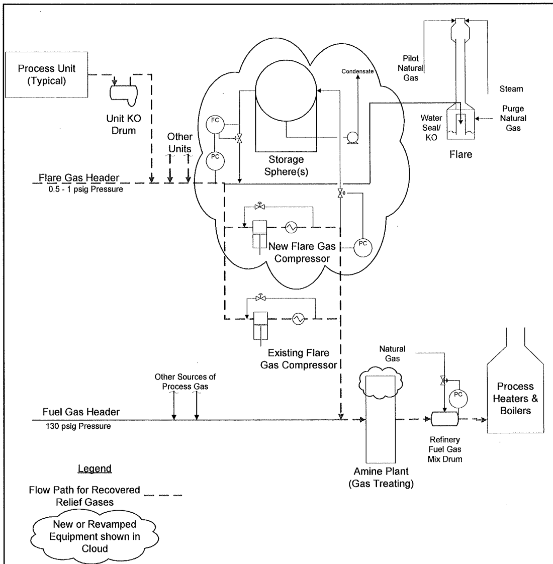
Figure 5-2, Flare Gas Recovery System with Additional Capacity
