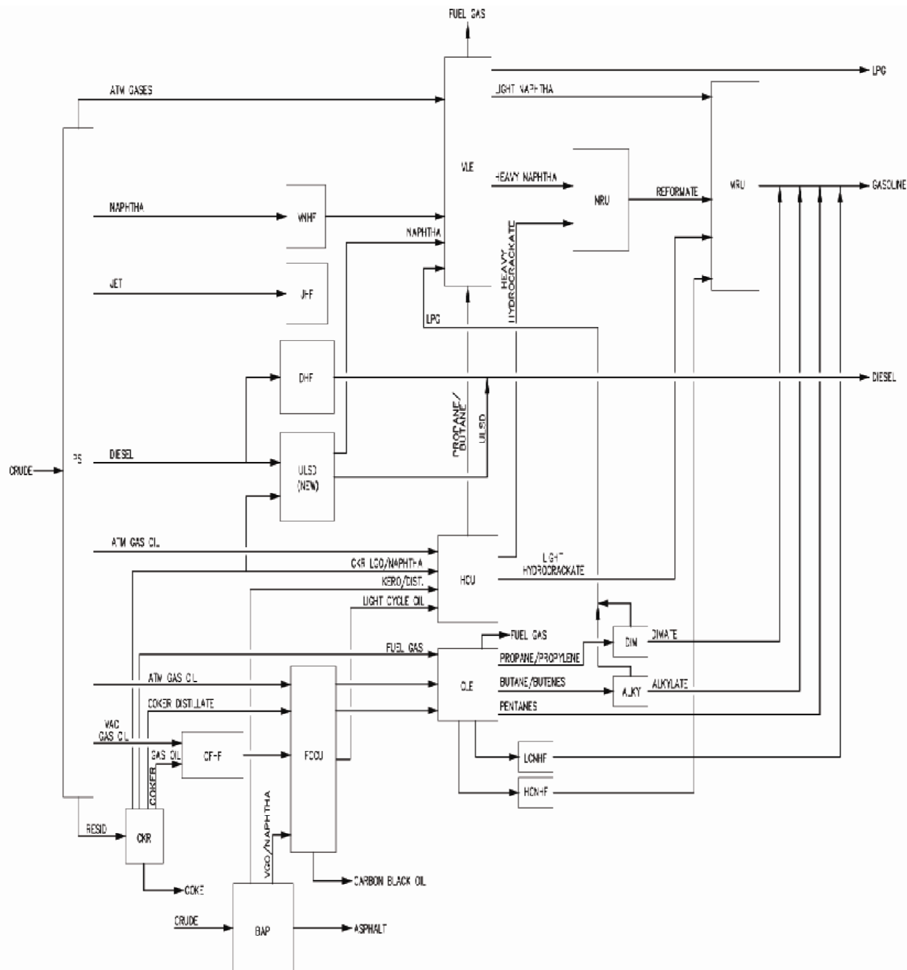
Figure 4 – Benicia Refinery Simplified Operations Flow Diagram
