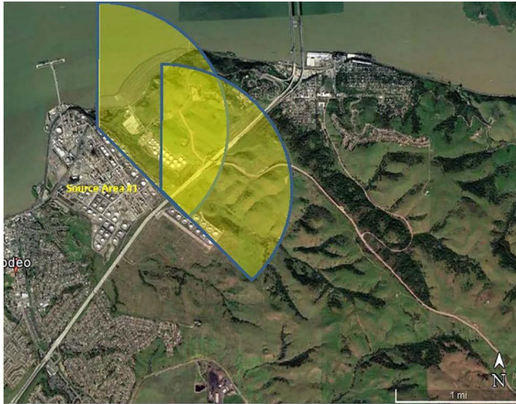
Figure 3 - Downwind Coverage Requirements – Source Area 1
