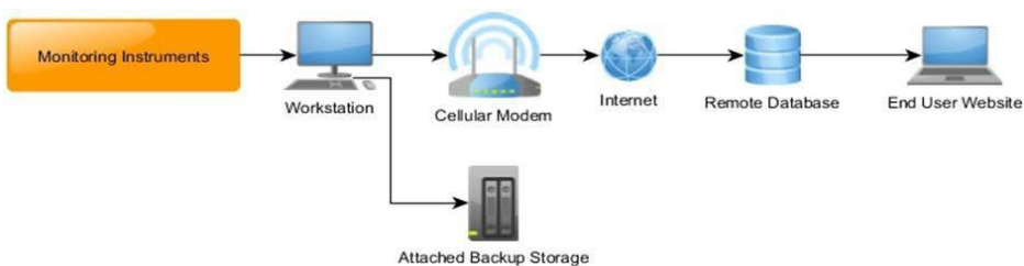
Figure 10 - Data Communication System
