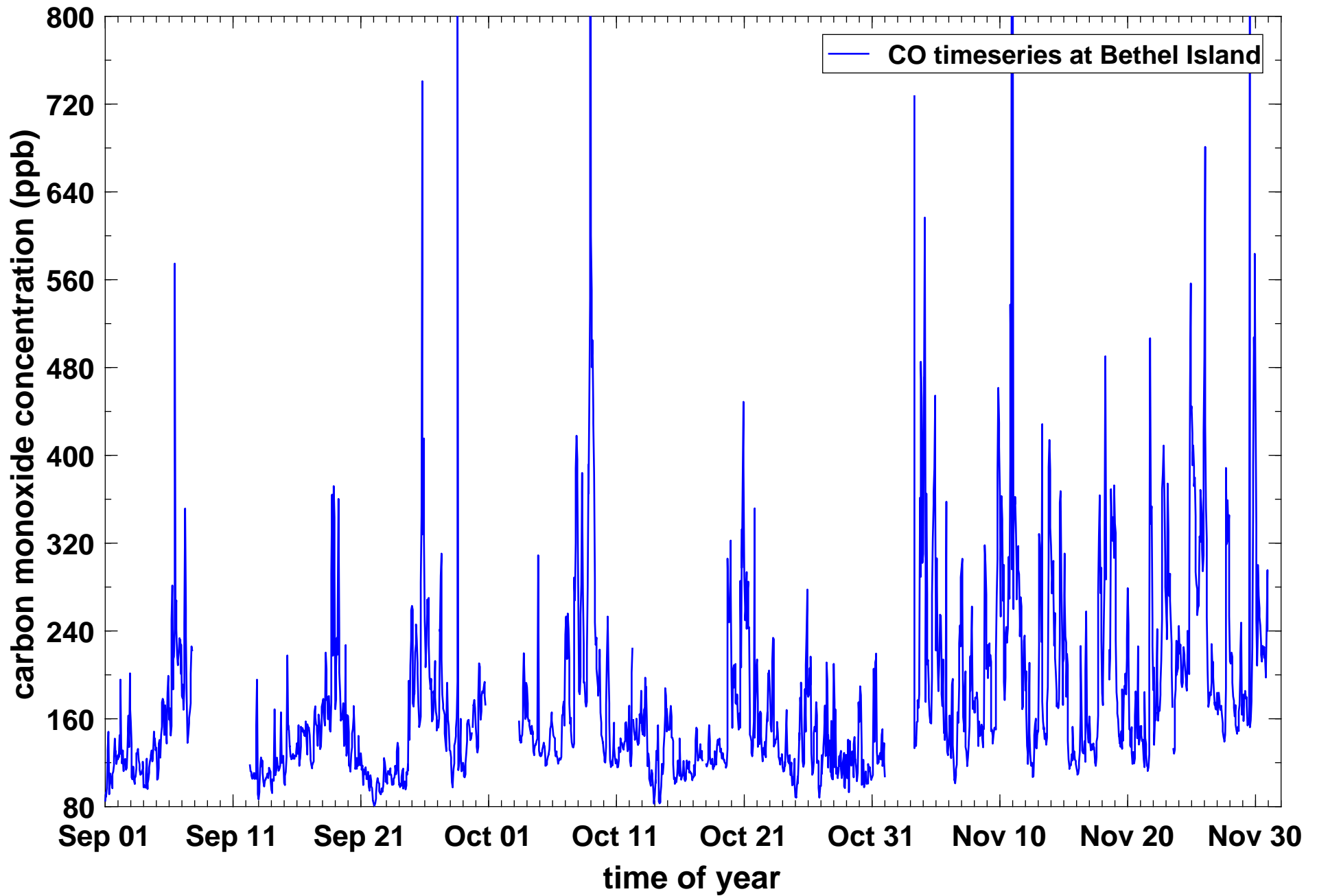
Timeseries of hourly CO concentrations (in ppb) at Bethel Island during fall 2016 (Sep 1 - Nov 30)..
