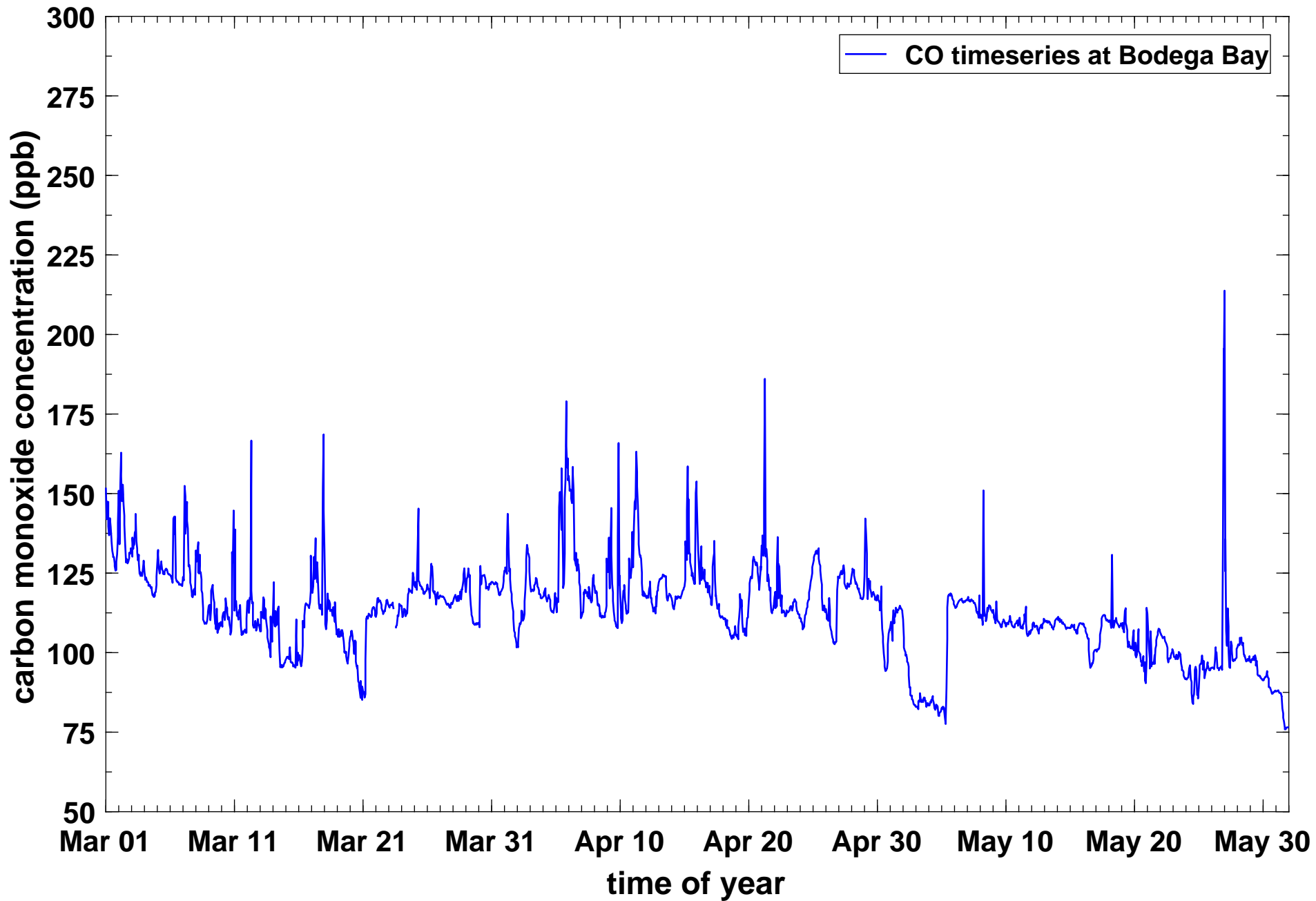
Timeseries of hourly CO concentrations (in ppb) at Bodega Bay during spring 2017 (Mar 1 - May 31).
