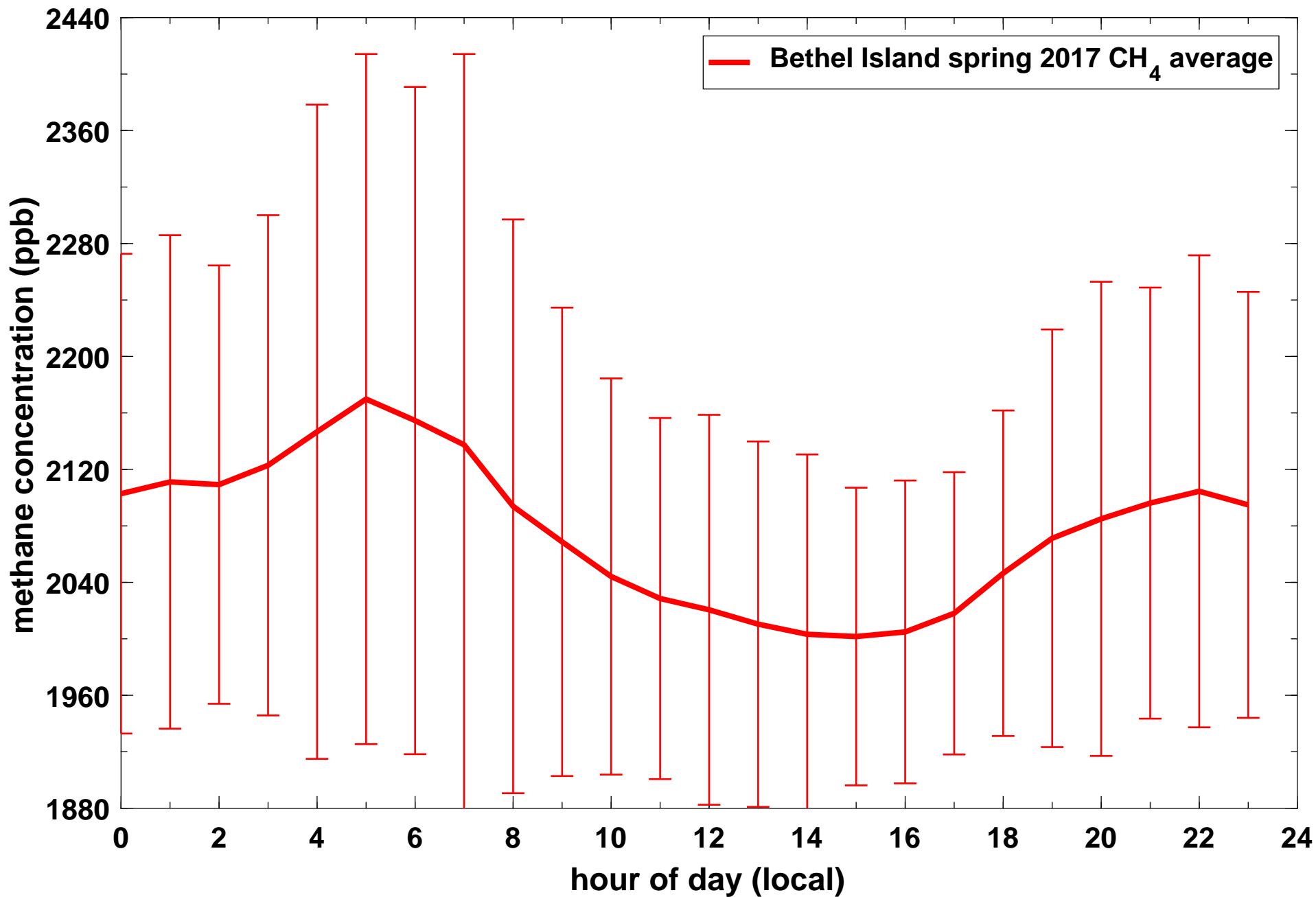
Average daily concentration profile of CH 4 (in ppb) at Bethel Island during spring 2017 (Mar 1 - May 31). The solid line denotes hourly averages for the entire season while the whiskers denote one standard deviation of the data values for each hour.
