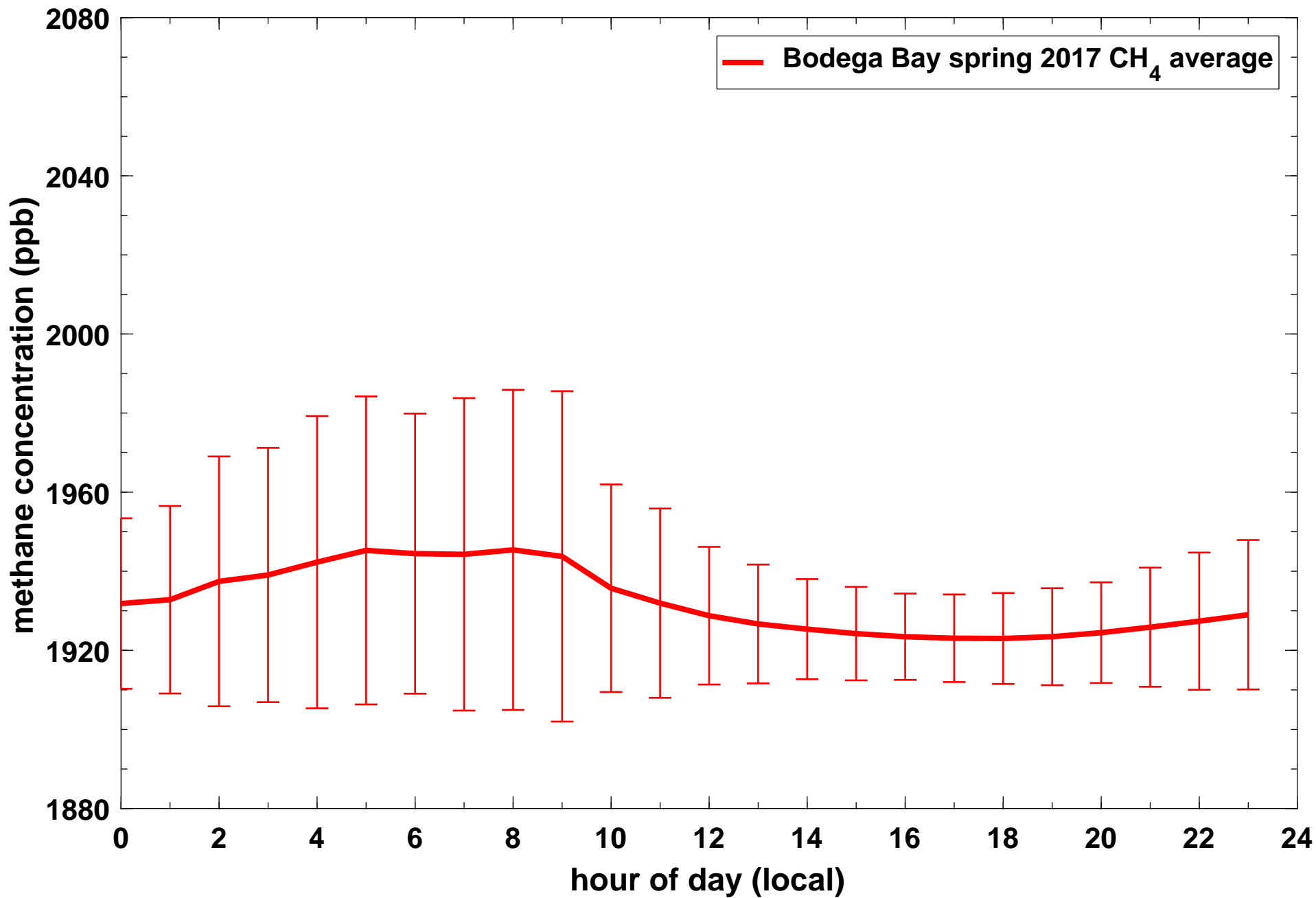
Average daily concentration profile of CH 4 (in ppb) at Bodega Bay during spring 2017 (Mar 1 - May 31). The solid line denotes hourly averages for the entire season while the whiskers denote one standard deviation of the data values for each hour.
