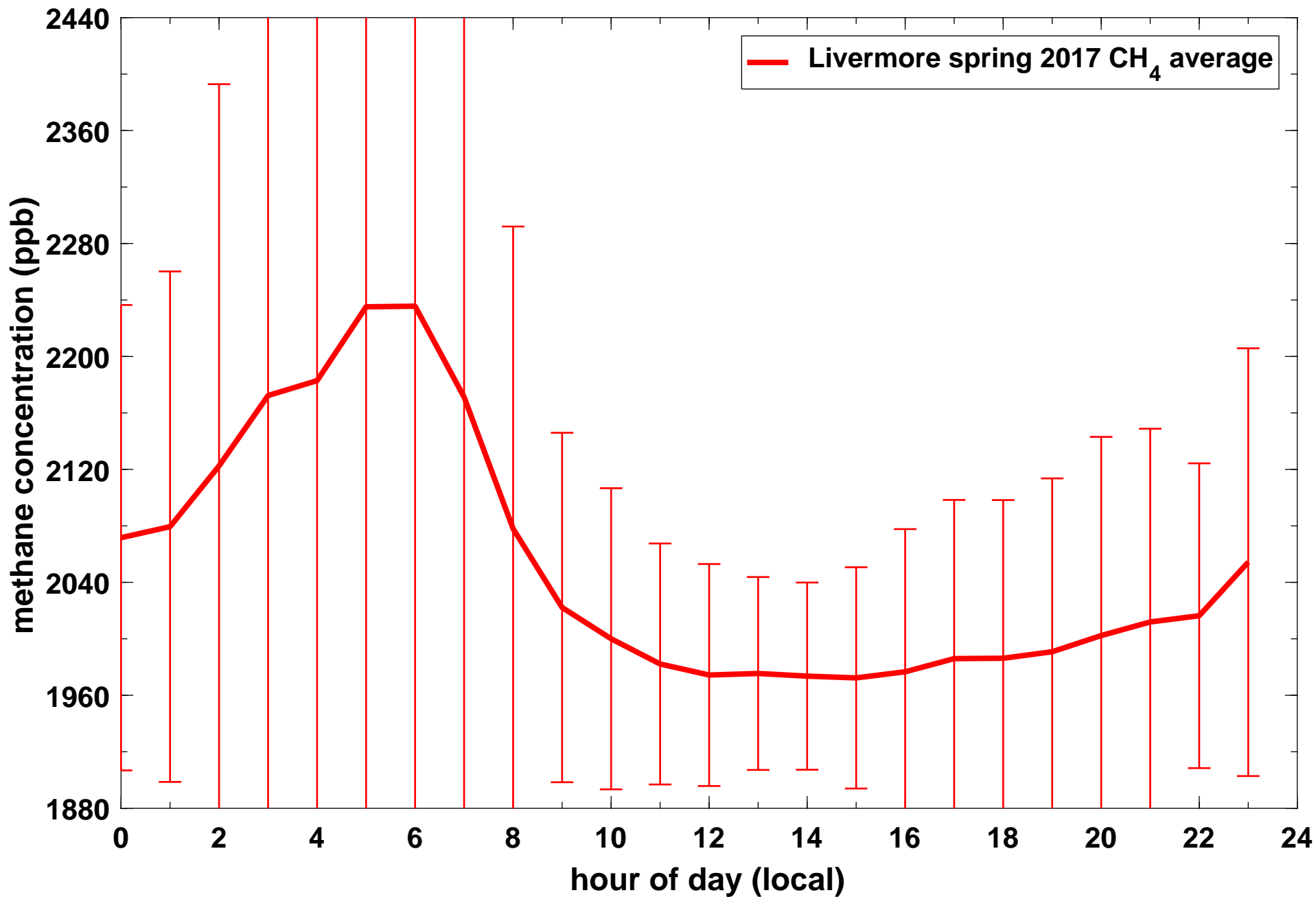
Average daily concentration profile of CH 4 (in ppb) at Livermore during spring 2017 (Mar 1 - May 31). The solid line denotes hourly averages for the entire season while the whiskers denote one standard deviation of the data values for each hour.
