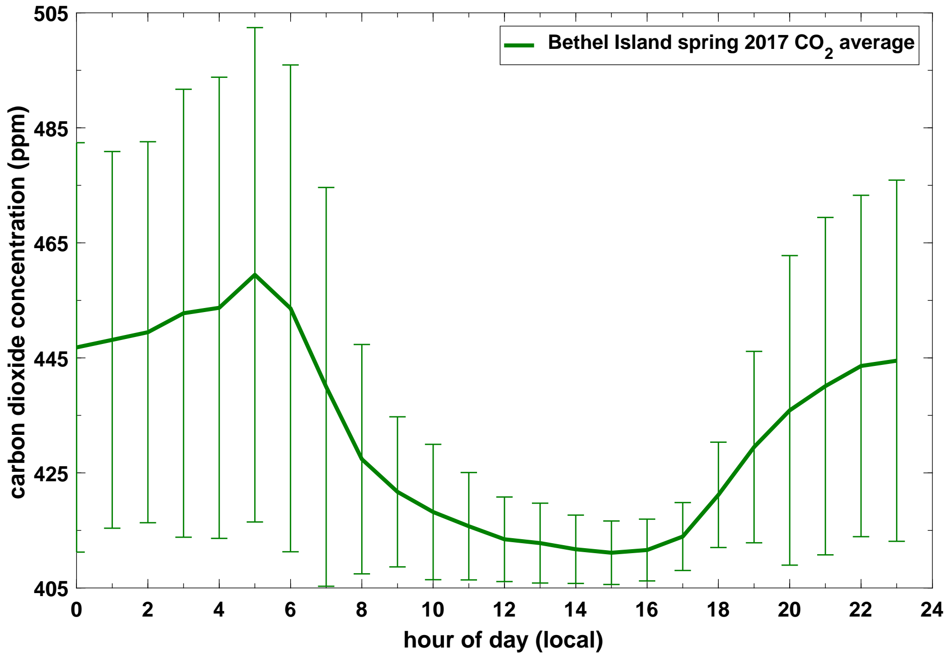
Average daily concentration profile of CO 2 (in ppm) at Bethel Island during spring 2017 (Mar 1 - May 31). The solid line denotes hourly averages for the entire season while the whiskers denote one standard deviation of the data values for each hour.
