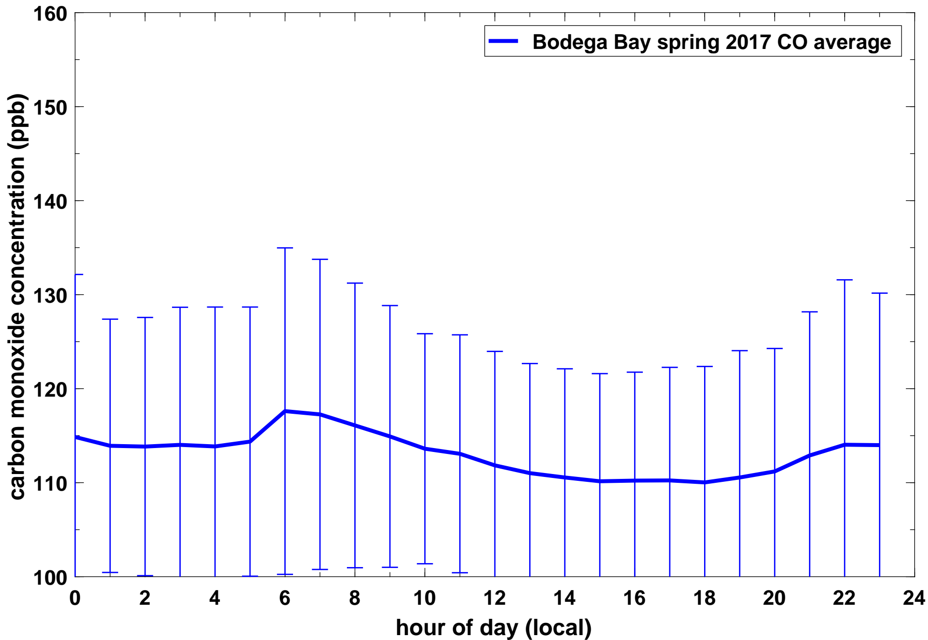
Average daily concentration profile of CO (in ppb) at Bodega Bay during spring 2017 (Mar 1 - May 31). The solid line denotes hourly averages for the entire season while the whiskers denote one standard deviation of the data values for each hour.
