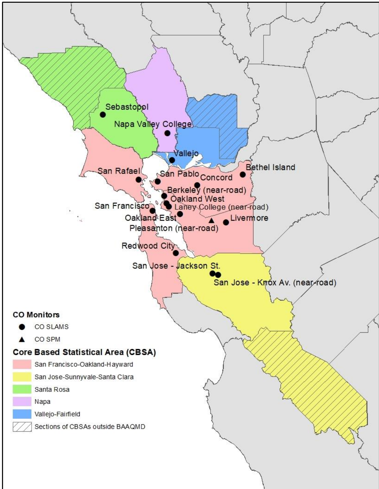
Figure 2-8. CO Monitoring in the San Francisco Bay Area in 2019
