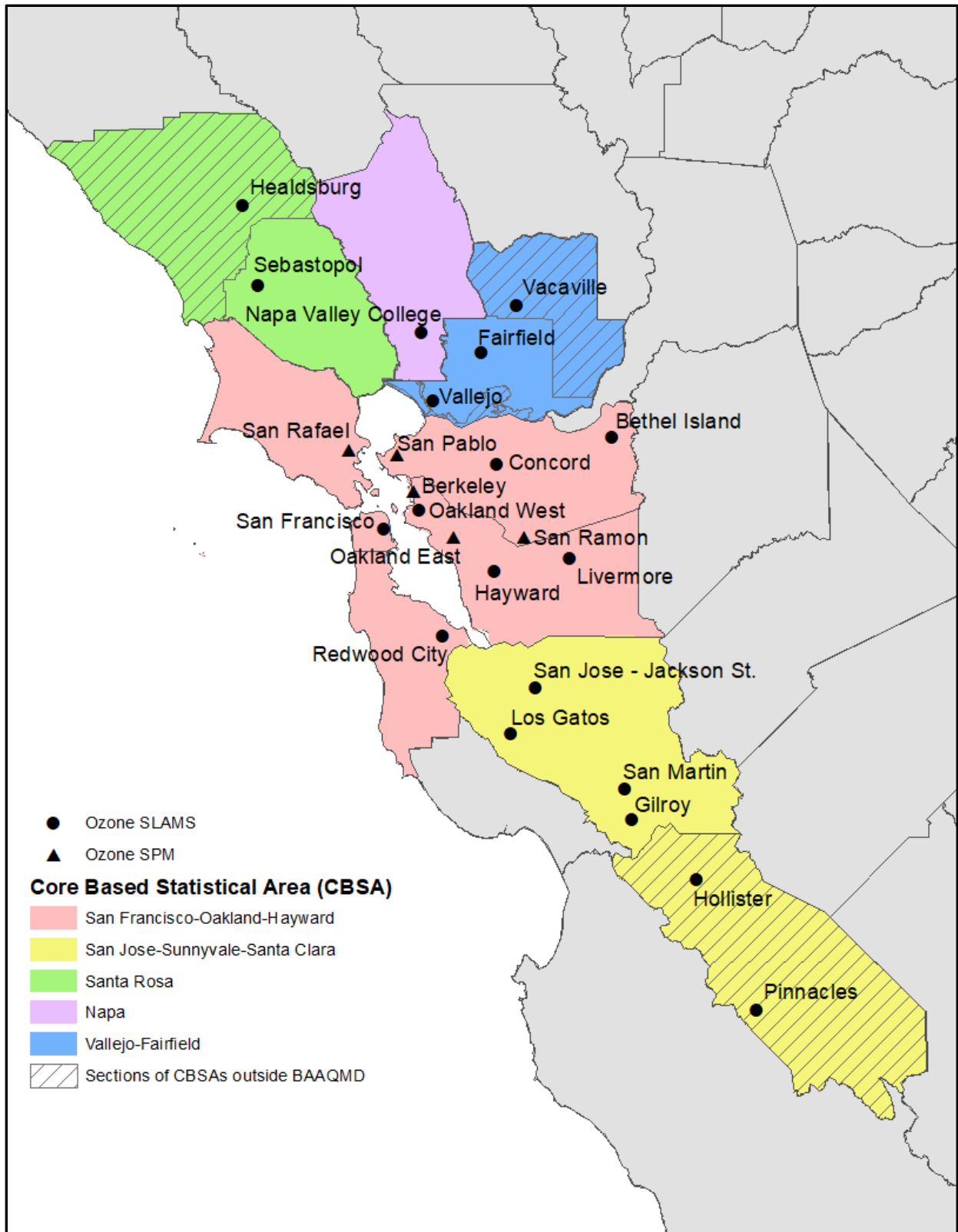
Figure 2-3. Ozone Monitoring in the San Francisco Bay Area in 2019
